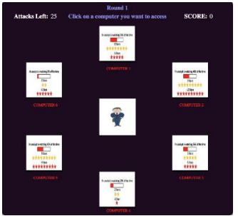
Signaling
